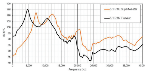
Response vs Frequency Direct into HiRes 711 (GRAS RA0403)
