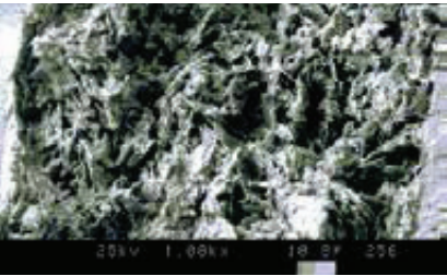
● Picture taken at 1,000x magnification using a SEM to demonstrate the fibrous nature of the FlexiCap™ termination that absorbs increased levels of mechanical stress.
