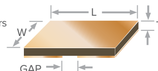
Split electrodes
