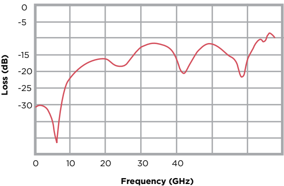
TYPICAL INSERTION LOSS (S21)
