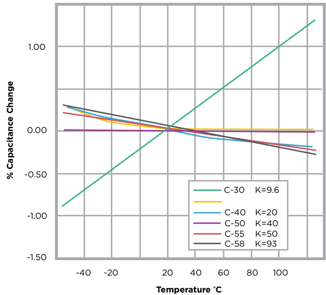
C-30/C-37/C-40/C-50/C-55/C-58
