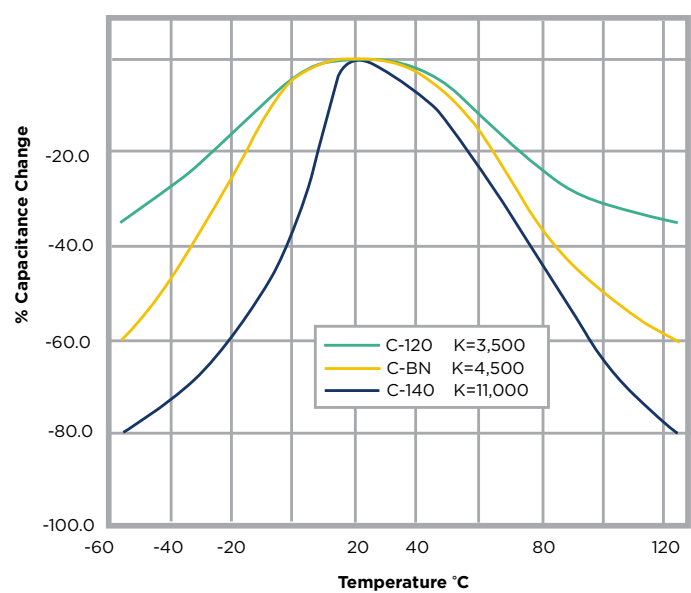
C-120/C-BN/C-140
