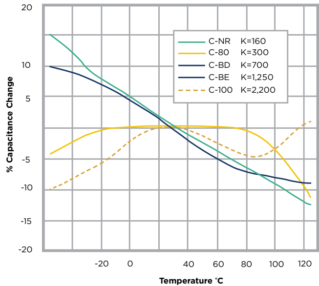
C-NR/C-80/C-BD (C-BE)/C-100
