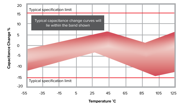
X7R (2R1)
