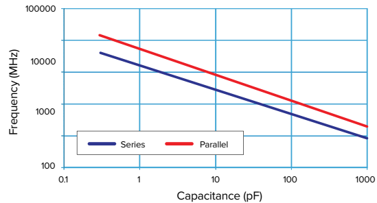
RESONANT FREQUENCY VS CAPACITANCE
