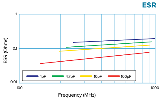
TYPICAL PERFORMANCE DATA — CHIP SIZE 0805 HIGH Q
