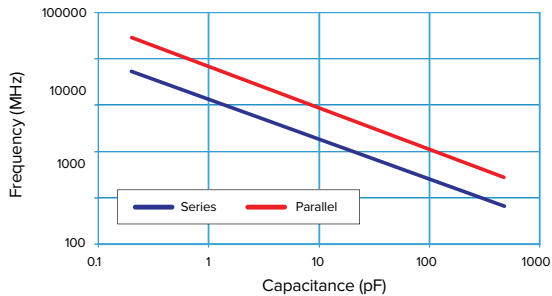
RESONANT FREQUENCY VS CAPACITANCE
