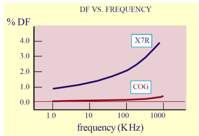
Figure 27. Dissipation Factor vs. Frequency
