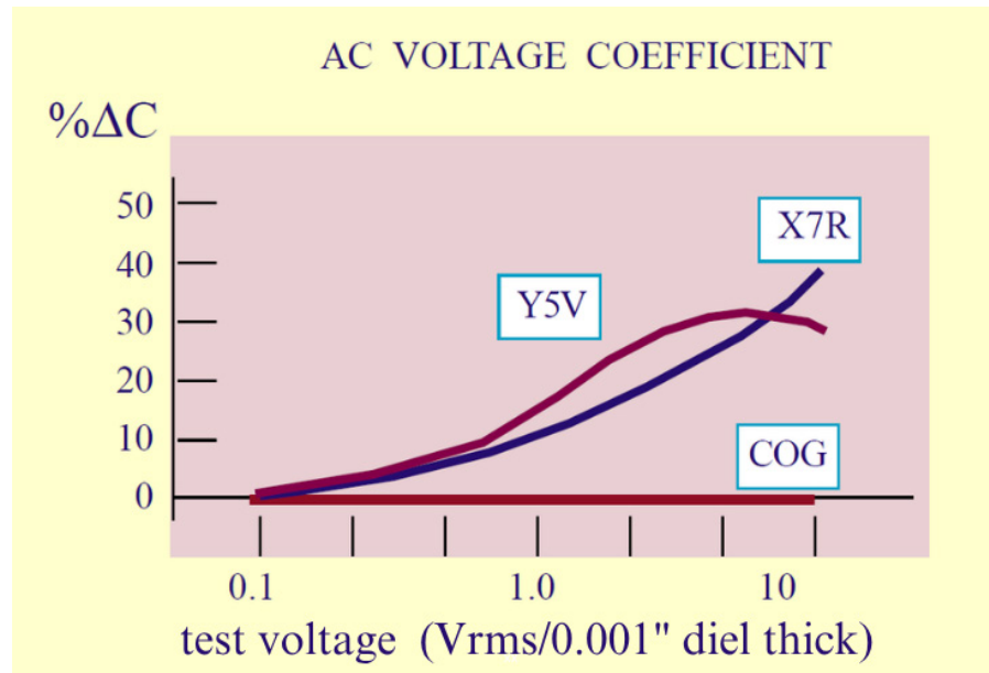
Figure 24. AC Voltage Coefficients
