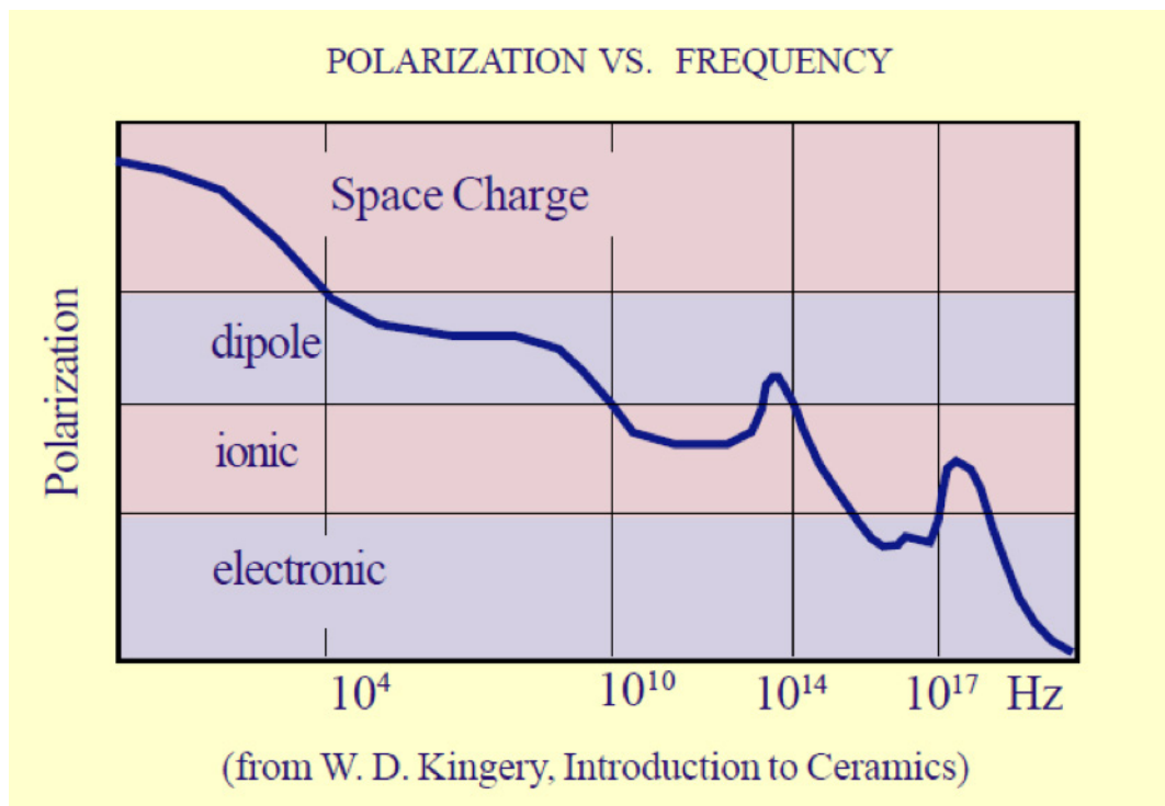
Figure 9: The Effect of Frequency on Polarization Mechanisms
