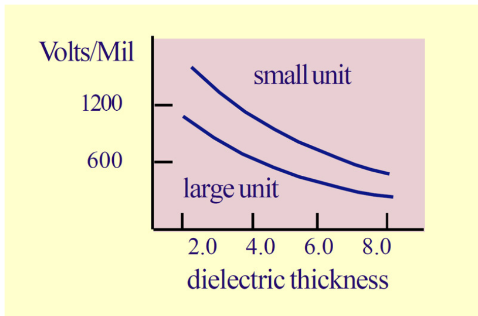
Figure 12: Dielectric Strength vs Dielectric Thickness
