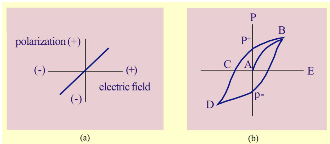
Figure 15. Polarization of Linear Dielectric (a) vs. Ferroelectric Dielectric (b)
