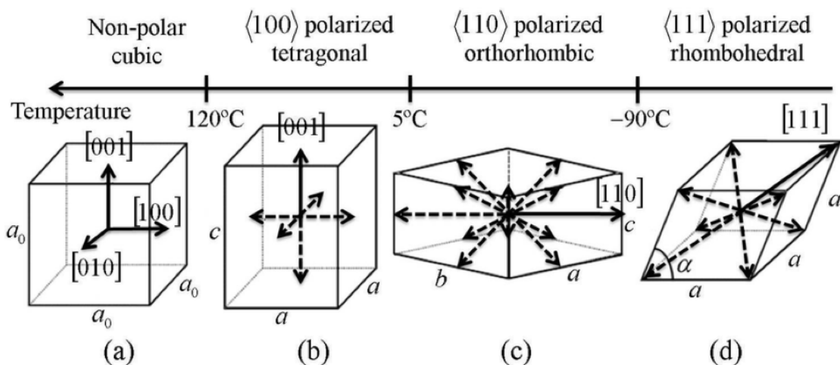
Figure 17. Phase Transformations of BaTiO 3 (source: University of Oxford)
