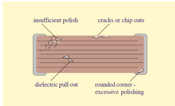
Figure 30. Sample preparation defects
