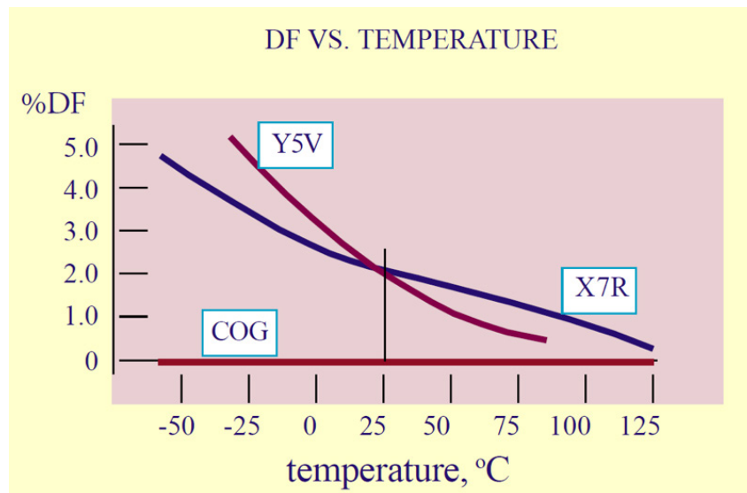
Figure 22. Dielectric Dissipation Factor Curves With Temperature
