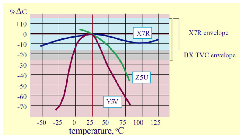
Figure 21. Temperature Coefficients of Ferroelectric Dielectrics
