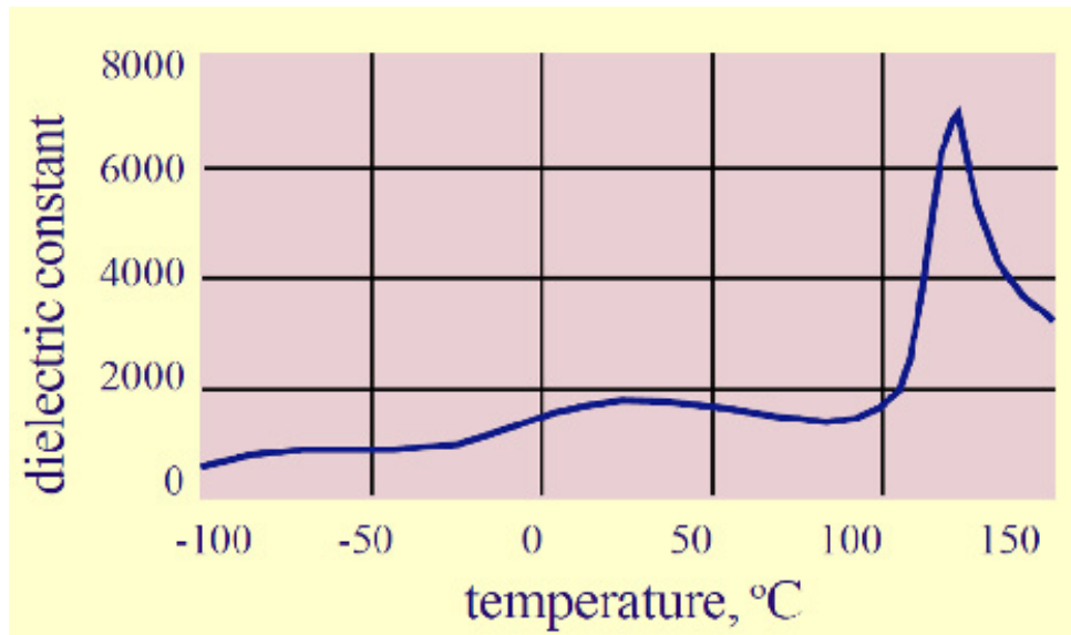
Figure 18. Changes in \text{BaTiO}_3 Dielectric Constant With Varying Temperature
