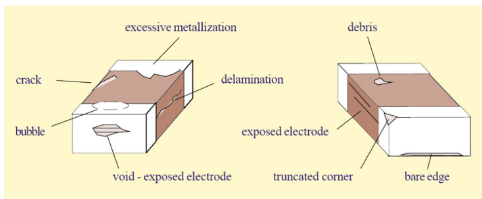
Figure 28. Visual Defects
