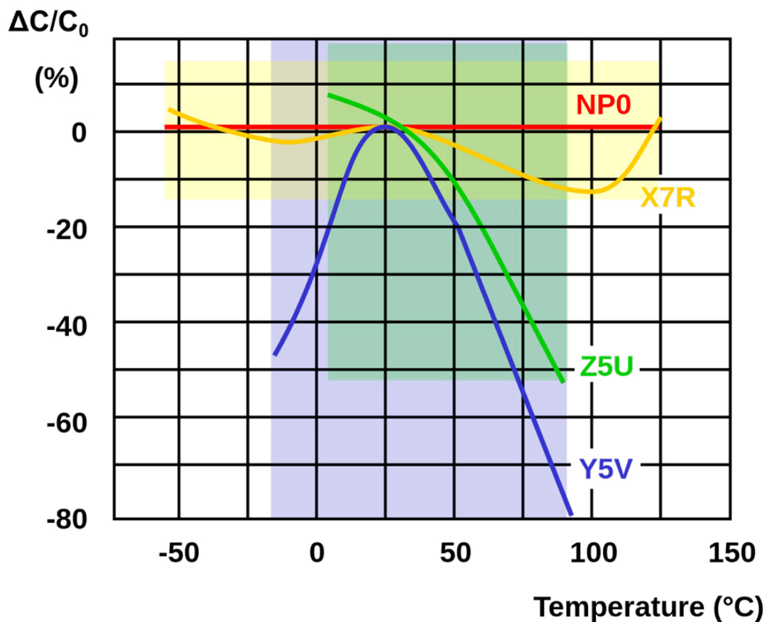
Figure 19. Capacitance Varying with Temperature for Different Capacitor Types (source: Wikipedia)
