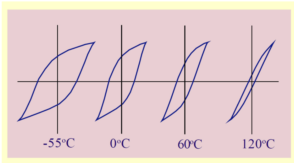
Figure 16: Hysteresis Loop at Various Temperatures
