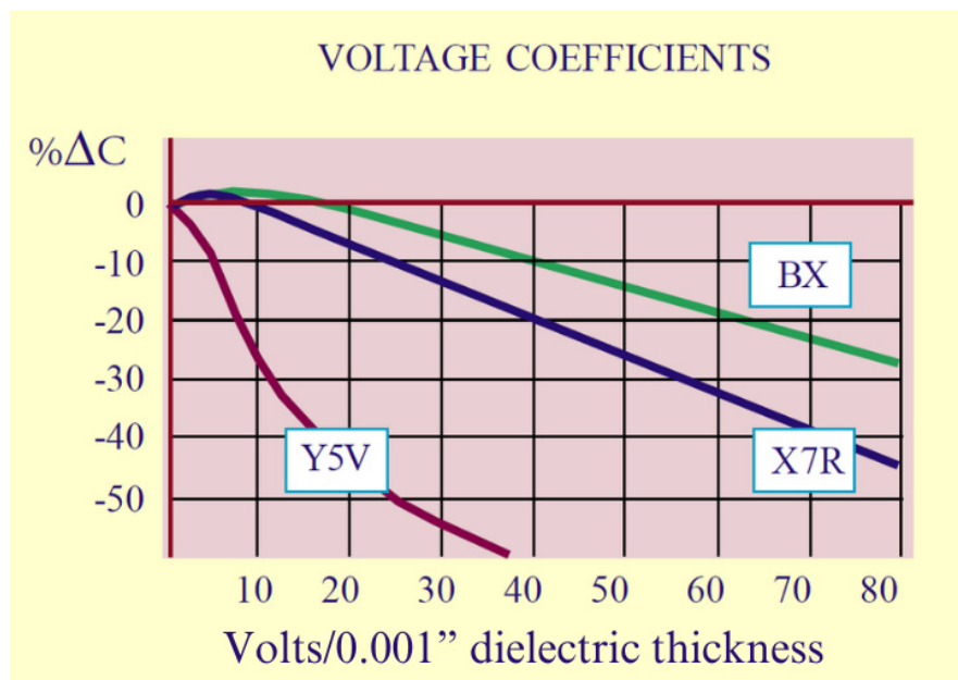
Figure 23. Voltage Coefficients for DC Bias
