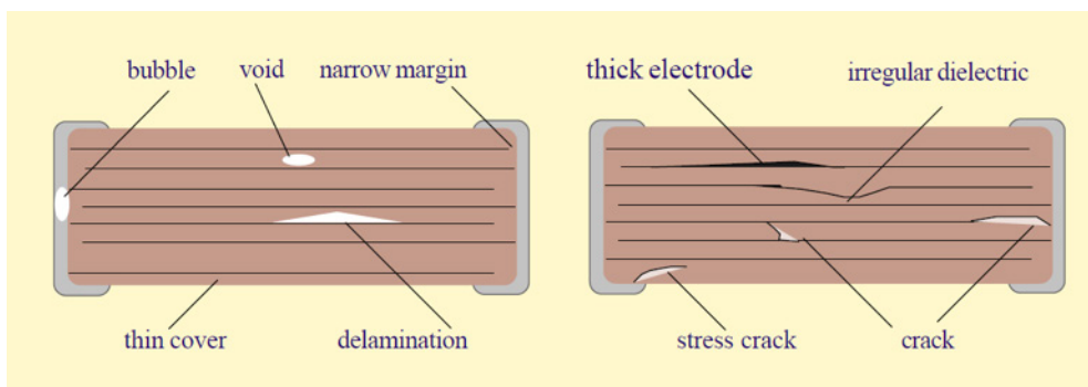
Figure 29. Microstructure Defects
