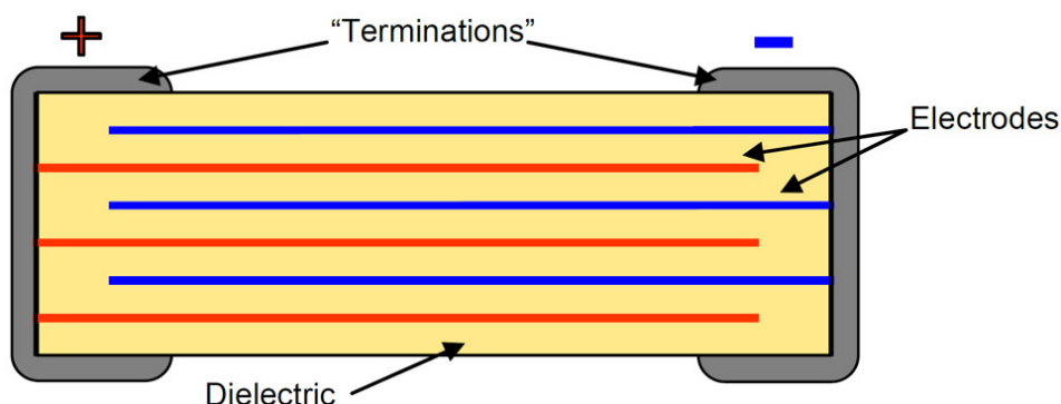
Figure 7: A Diagram of an MLCC
