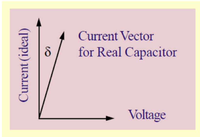
Figure 31. Loss Tangent in a Real-World Capacitor
