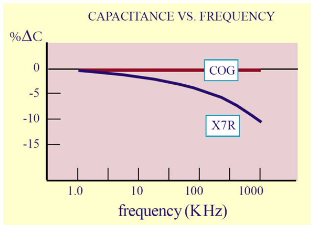
Figure 26. Capacitance vs. Frequency
