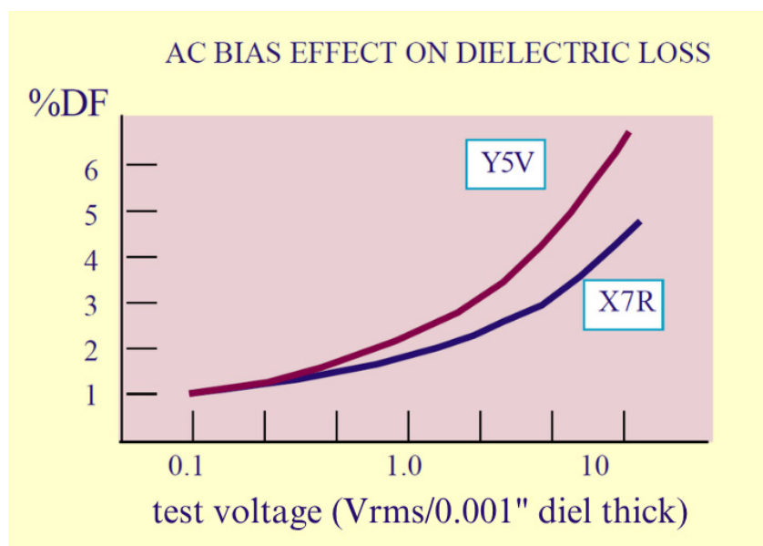
Figure 25. AC Bias Effect on Dielectric Loss
