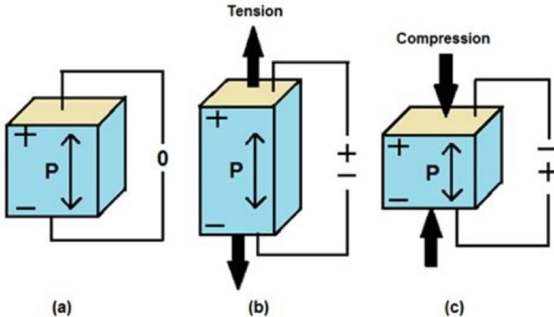
Figure 14: Different Piezoelectric Responses to Applied Mechanical Stress (source: ResearchGate)
