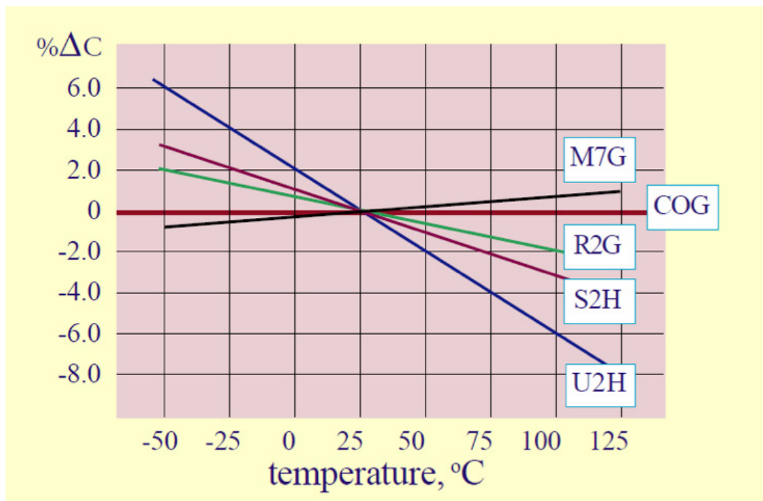
Figure 20. Temperature Coefficients of Linear Dielectrics
