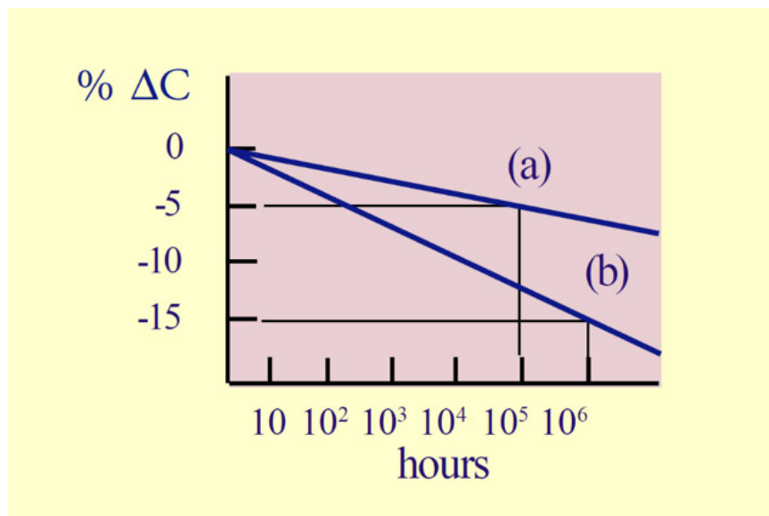
Figure 13: Ferroelectric Aging Shown as Percent Change in Capacitance (%ΔC) Over Time
