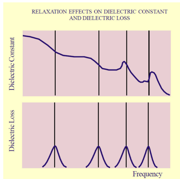
Figure 11: Changes in Dielectric Constant and Dielectric Loss Caused by Frequency
