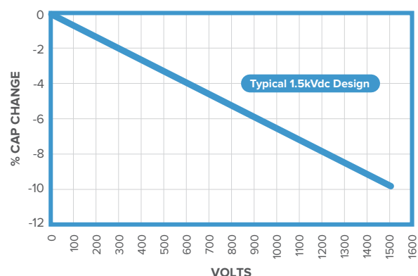
Voltage-capacitance coefficient
